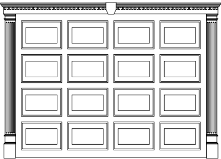
Garage Door Surround with 6" Header Up to 144" Classic Dentil Profile
